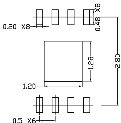
TYPICAL RECOMMENDED STENCIL
